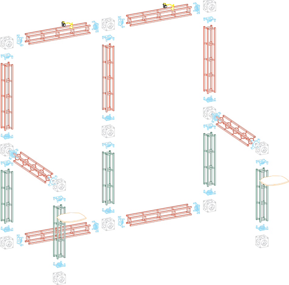
Parts exploded
